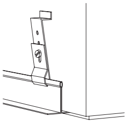
T-BAR BRACKET DETAIL
