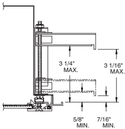
FLANGE SWING BAR DETAIL
