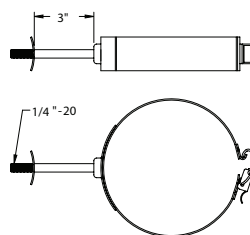
QUICK RELEASE WALL MOUNTING BRACKET (QWM)
