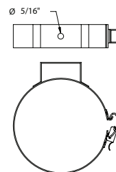
QUICK RELEASE CABLE MOUNTING BRACKET (QCM)
