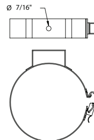
QUICK RELEASE CABLE MOUNTING BRACKET (QCM)
