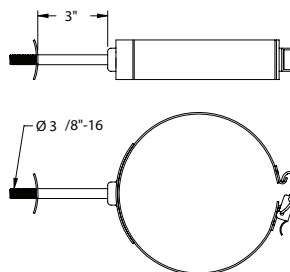
QUICK RELEASE WALL MOUNTING BRACKET (QWM)
